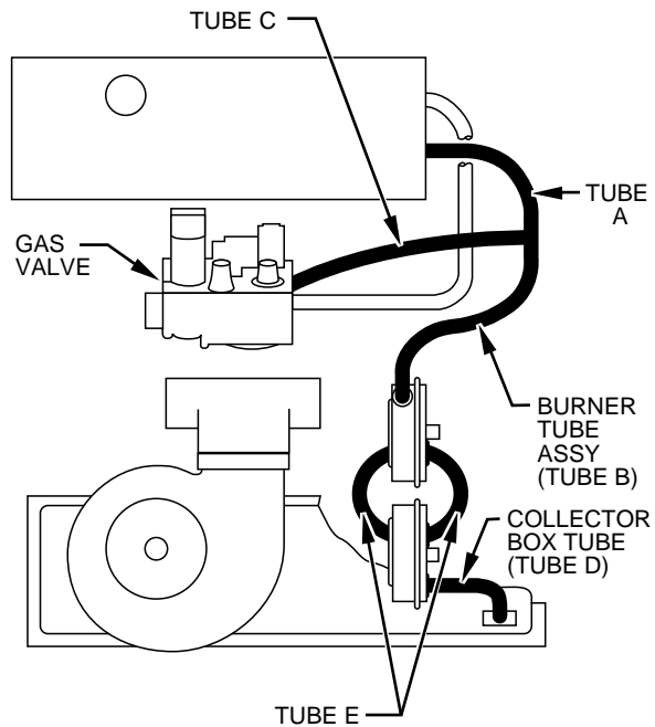
Fig. 3—Pressure Tube Connection Diagram for Models 398BAZ and 58SXB Furnaces
